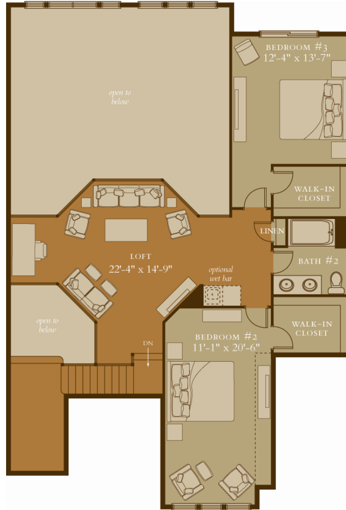
UPPER LEVEL
